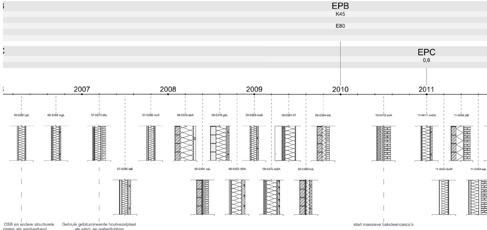
Iterations on hybrid wall compositions from "30 Ways To Build a Wall". N.Claeys, UGent 2019
